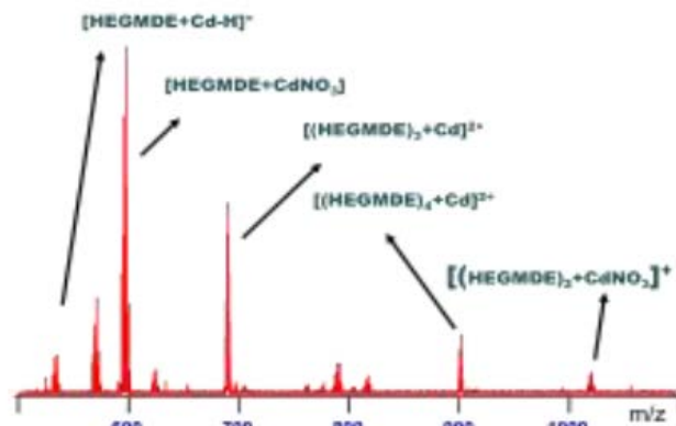
Figure 1. ESI-FT/ICR mass spectrum of HEGMDE+Cd(NO 3 ) 2 .4H 2 O.
