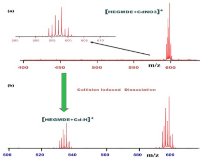
Figure 4. ORI-ESI-FT/ICR CID mass spectra of HEGMDE+Cd(NO 3 ) 2 .4H 2 O.
