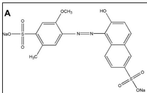
Fig. 1 Chemical structure of Allura Red AC [4].
