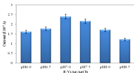
Fig. 3 The relationship between the oxidation peak current and pH of Tris-HCl buffer with MB in solution containing 10 ppm of Allura Red.
