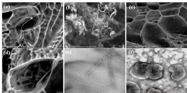
Fig. 2 SEM image of the (a) CHIT, (b) MWCNTs, (c) CHIT/ZnONPs, (d) CHIT/ZnONPs/MWCNTs and, TEM image of (e) MWCNTs, (f) CHIT/ZnONPs
