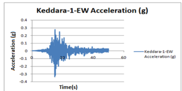
Fig. 2: E-W component of the Boumerdes earthquake acceleration recorded at station 1 in Keddara (PGA = 0.33g at 15.195s)
