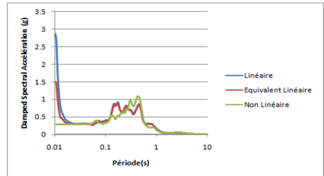
Fig. 5: Damped response acceleration spectra of the Foes site
