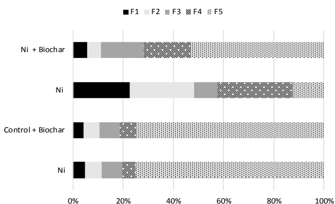
Fig. 6. Distribution of Ni fractions in control and Ni-treated soil by biochar applications
