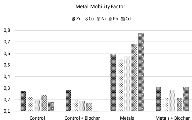
Fig 9. Change of metal mobility factor (MF) in control and metal treated soil by biochar applications
