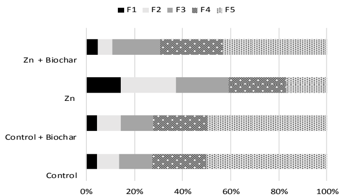
Fig 4. Distribution of Zn fractions in control and Zn-treated soil by biochar applications
